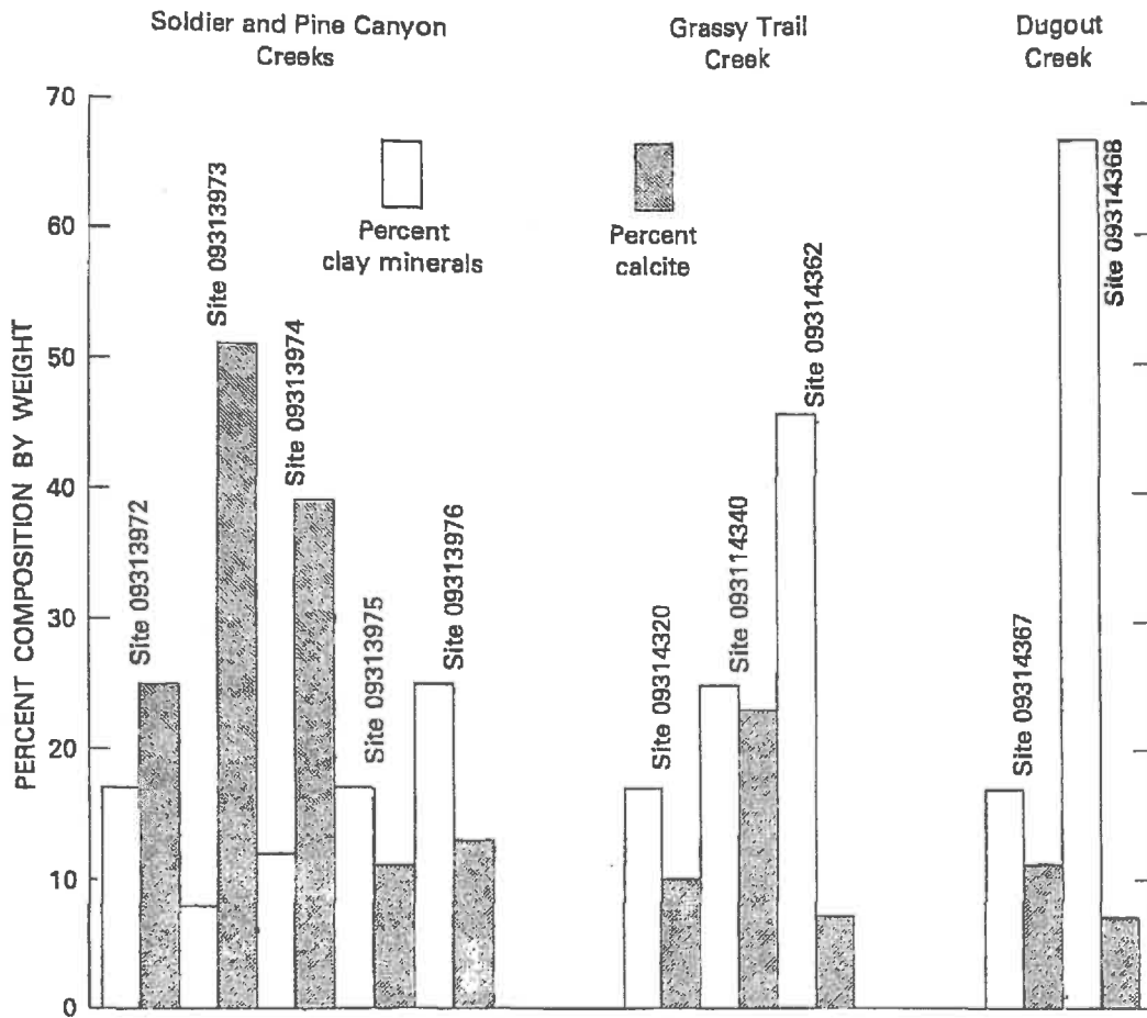
FIGURE 9.—Mineralogic composition of bed material at sites on selected streams.
