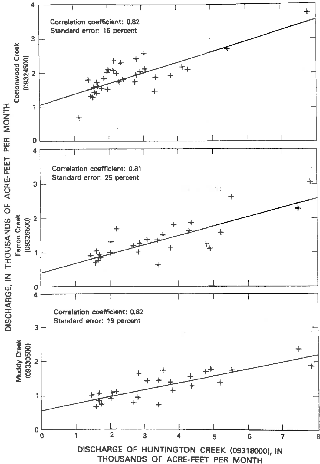
FIGURE 6.—Relationship of September flows at Huntington Creek to sites on Cottonwood, Ferron, and Muddy Creeks. Numbers in parentheses are gaging-station locations.
